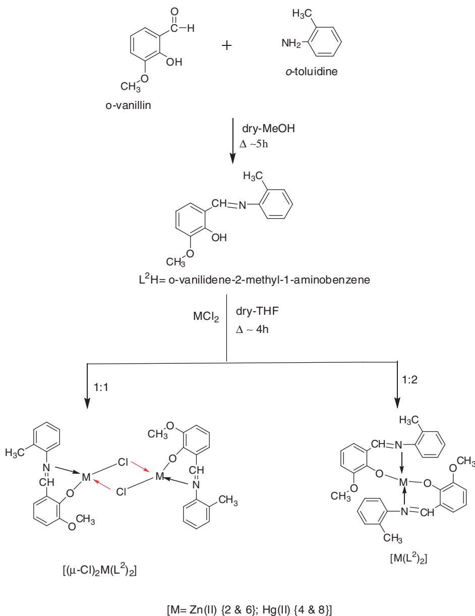
Scheme 2. Synthesis of L^2H and complexes.
