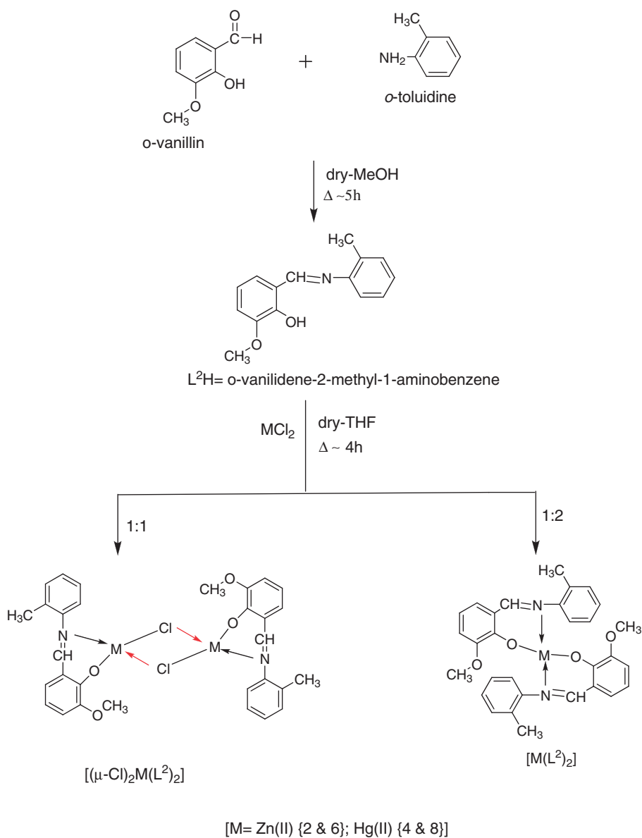
Scheme 1. Synthesis of \text{L}^1\text{H} and complexes.
